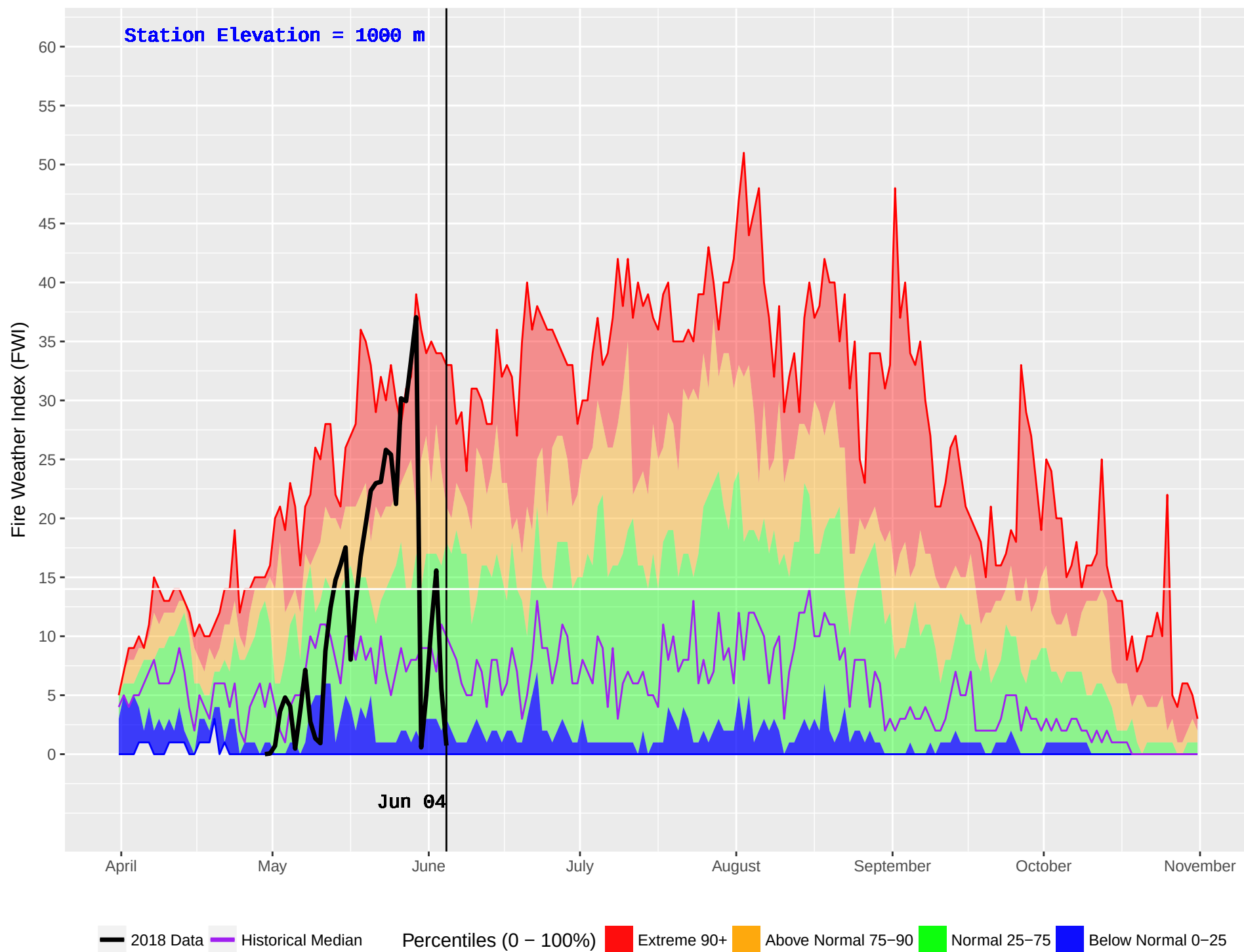
SUCCOUR CREEK (374) : Historical (1986–2016) and Current (2018) Noon Fire Weather Index (FWI)
