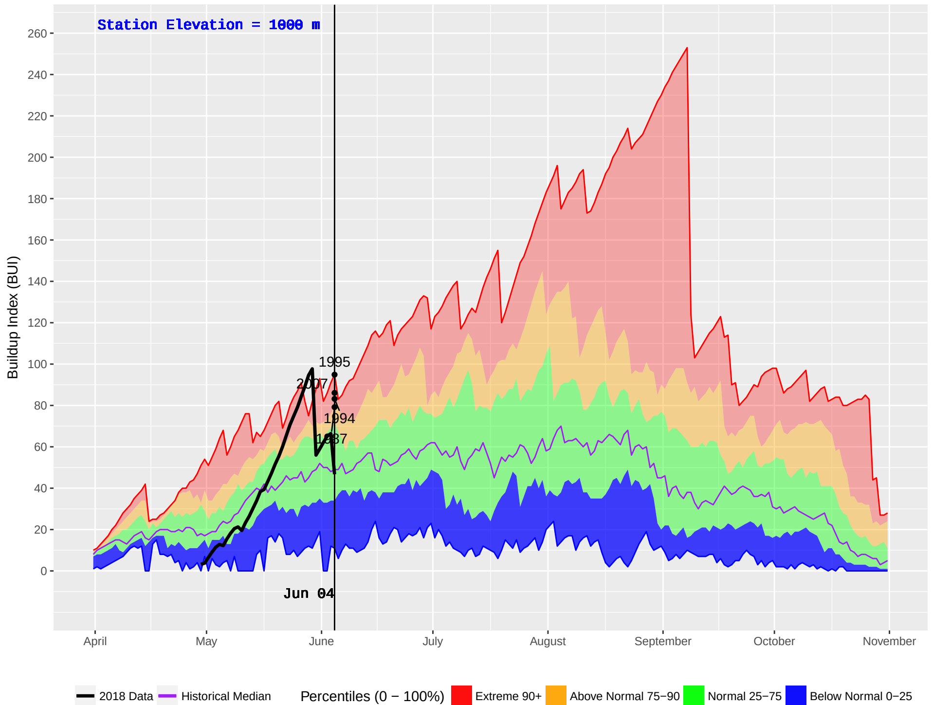
SUCCOUR CREEK (374) : Historical (1986–2016) and Current (2018) Noon Buildup Index (BUI)
