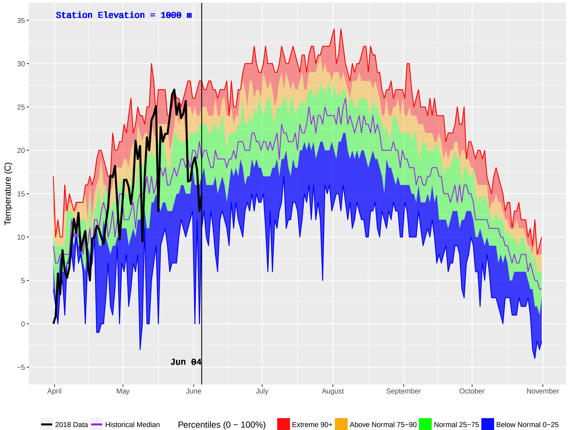
SUCCOUR CREEK (374) : Historical (1986–2016) and Current (2018) Noon Temperature
